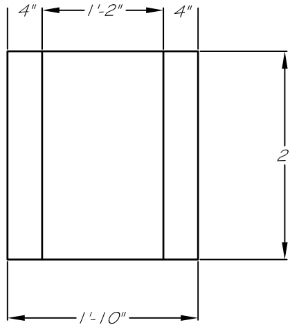
SECTION VIEW
