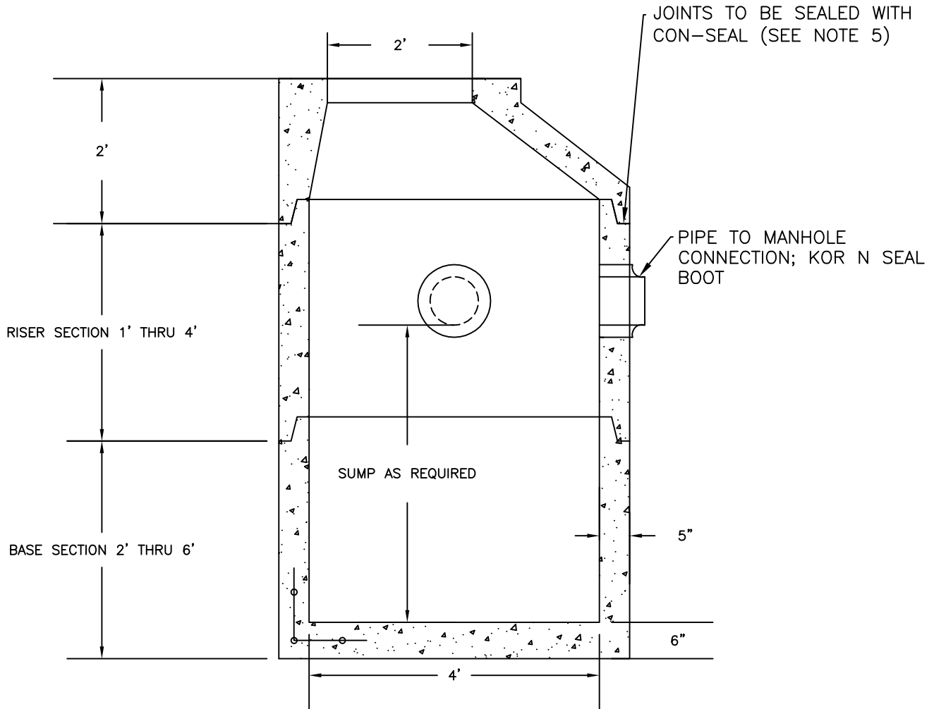
SECTION VIEW
