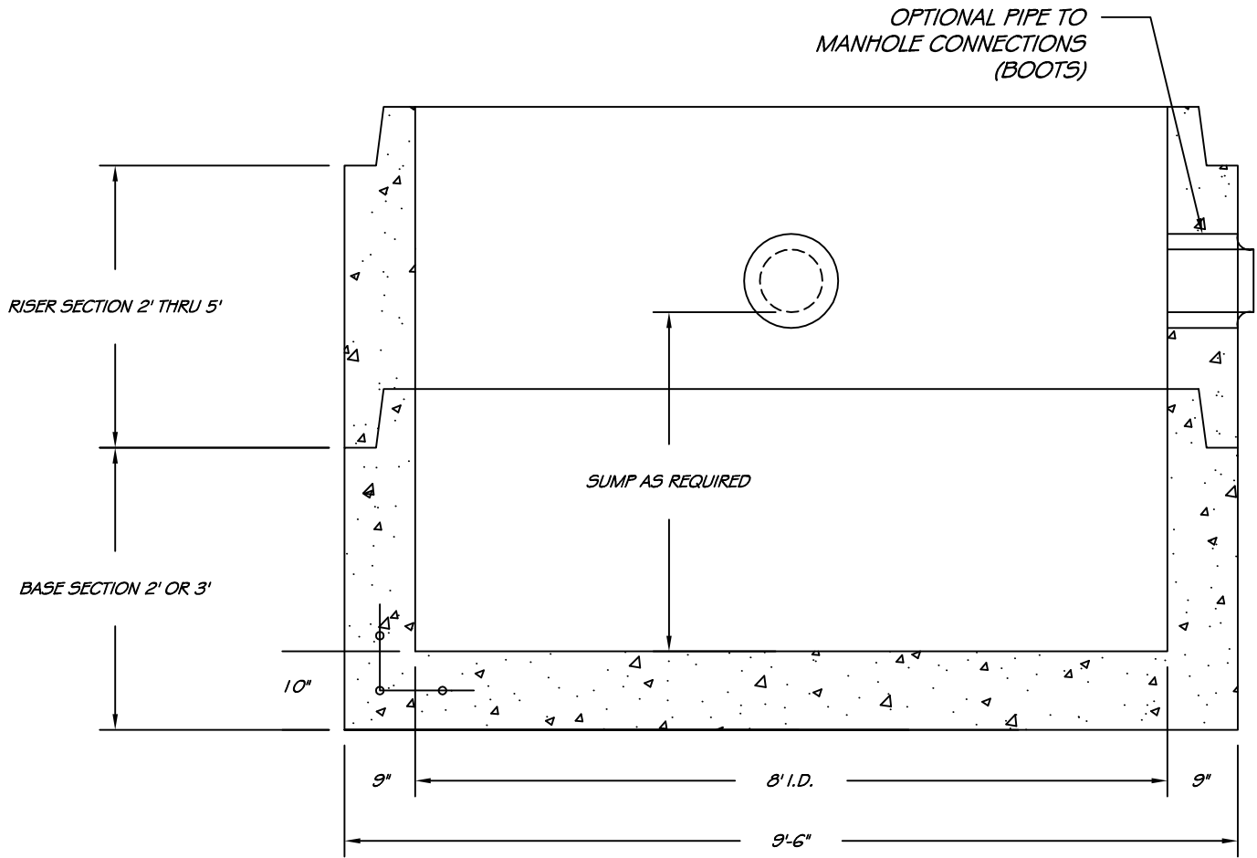
SECTION VIEW
