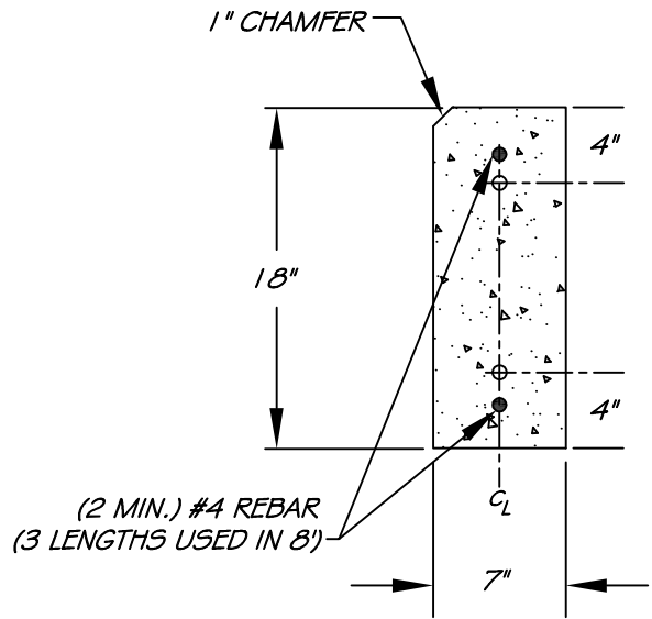
SECTION VIEW
