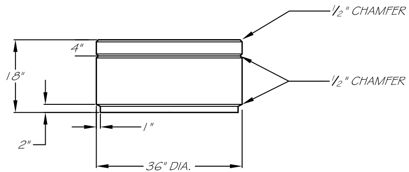
ELEVATION VIEW
