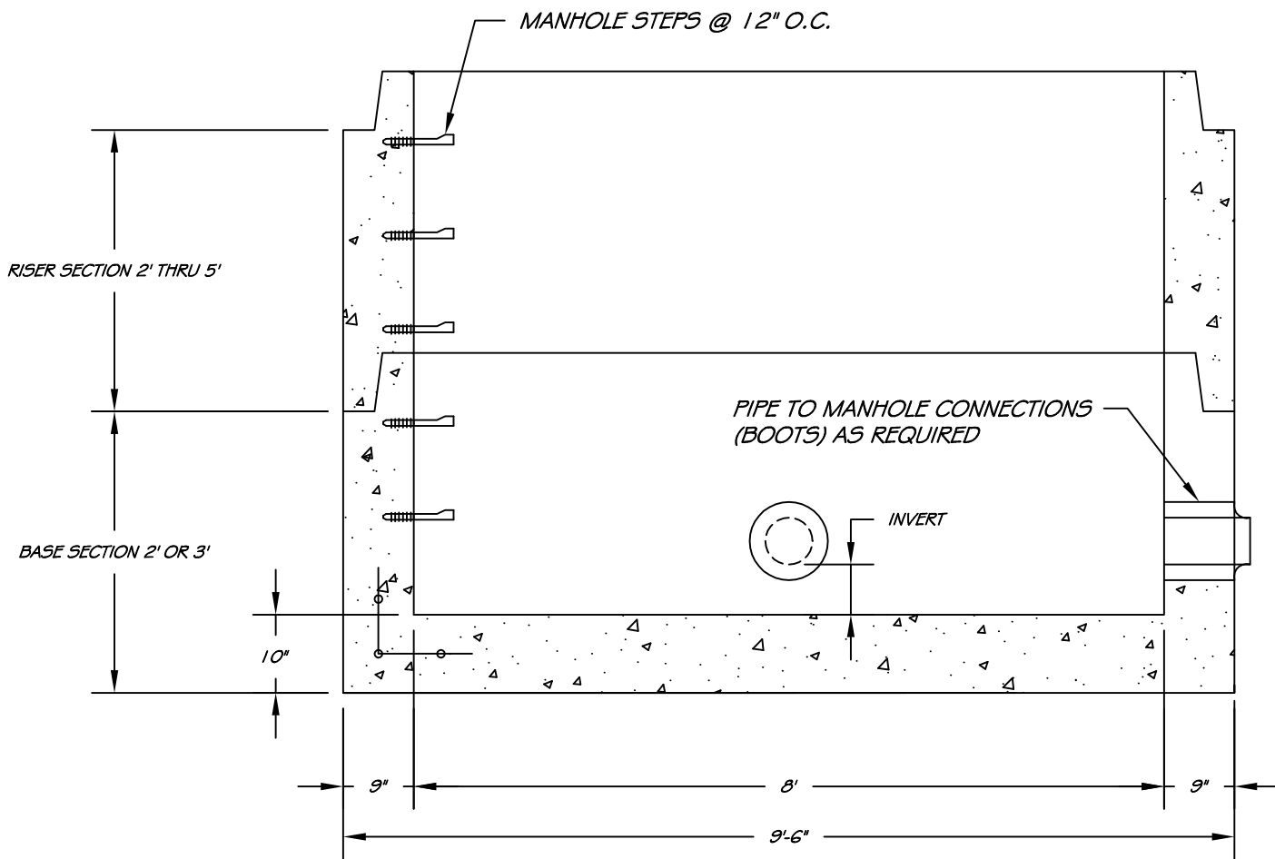
SECTION VIEW
