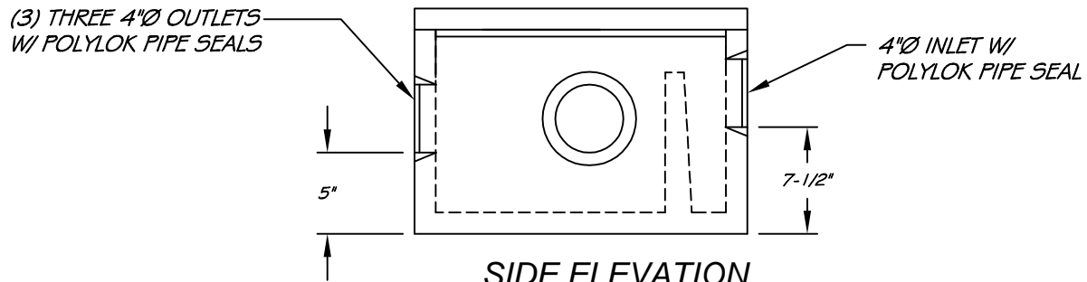
SIDE ELEVATION
