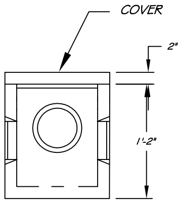
END VIEW
