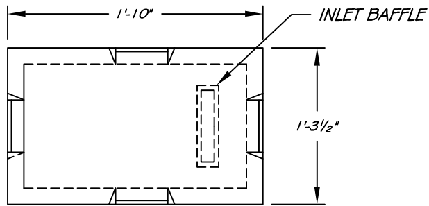
PLAN VIEW (W/O COVER)
