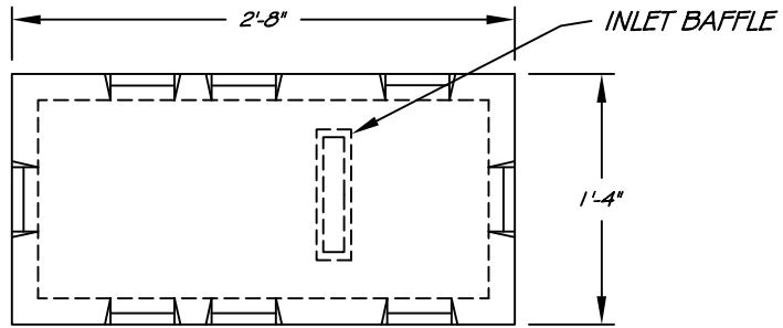
PLAN VIEW (W/O COVER)
