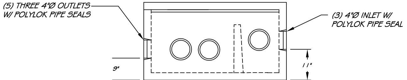
SIDE ELEVATION
