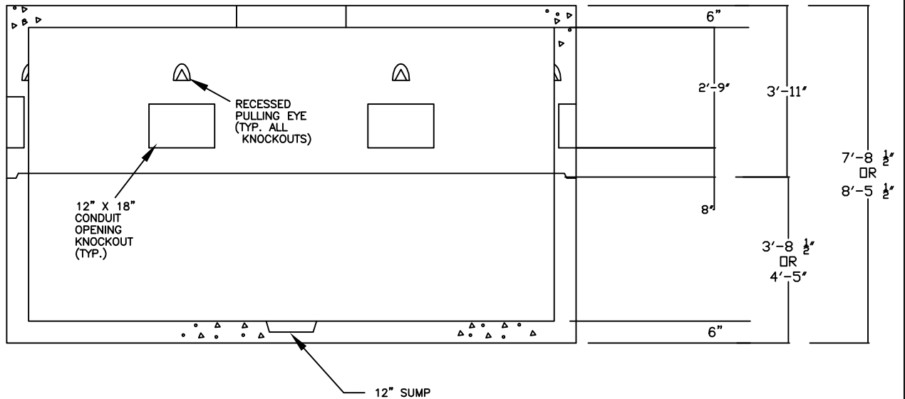
SECTION VIEW
