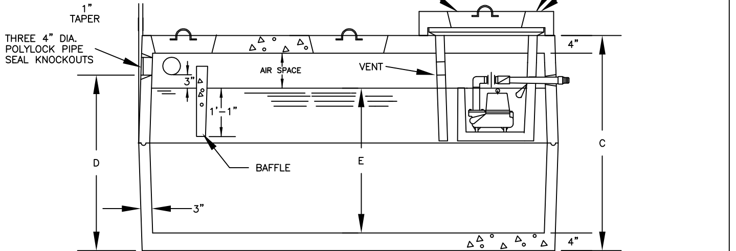
SIDE ELEV. VIEW SECTIONED
