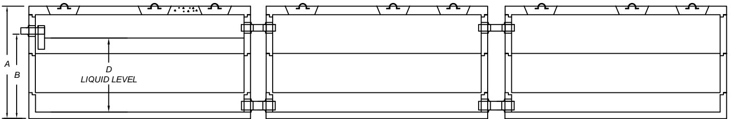
SECTION VIEW
