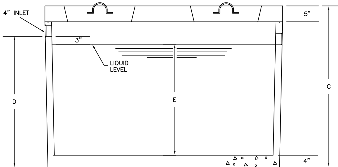
SIDE ELEV. VIEW SECTIONED
