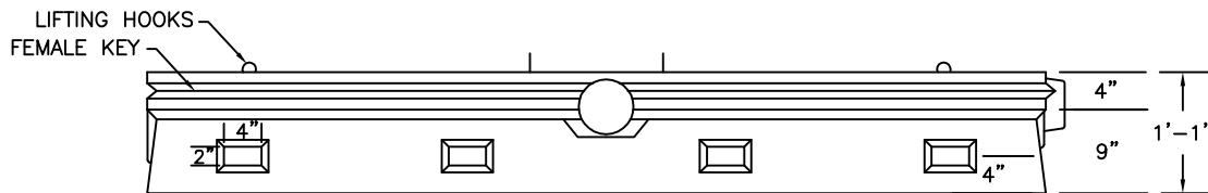
SIDE VIEW
