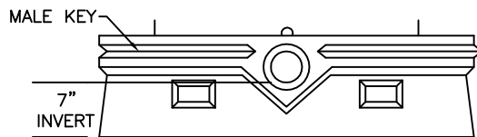
RIGHT END VIEW
