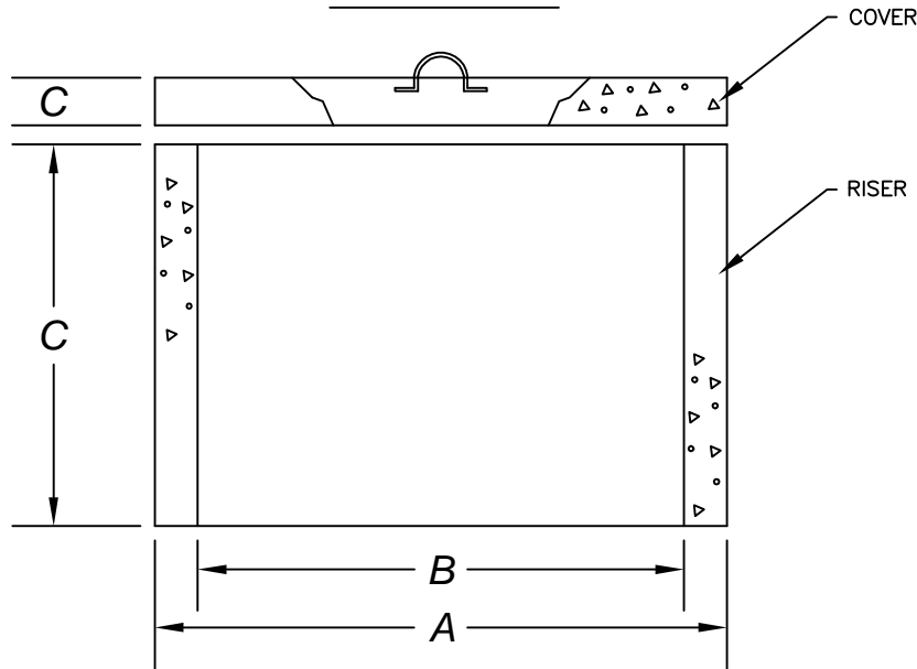
SIDE ELEV. VIEW SECTIONED
