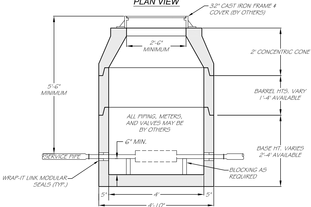
SECTION VIEW
