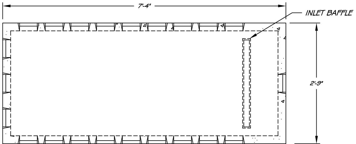
PLAN VIEW (W/O COVER)
